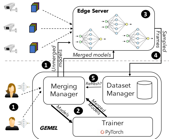
Figure 8: GEMEL architecture.
